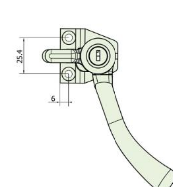
2-Hole Backplate Dimensions
