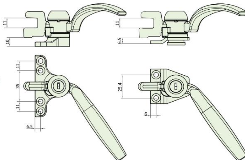
4-Hole Backplate Dimensions
