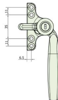
4 Hole Backplate Dimensions
