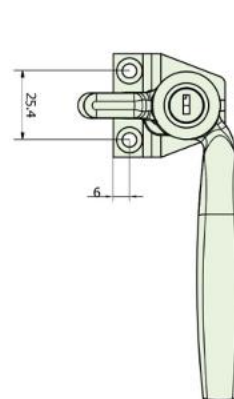
2 Hole Backplate Dimensions
