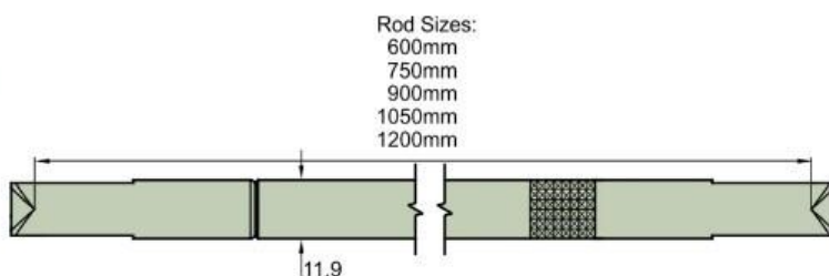
B646 Connecting Rod with connector fitted
