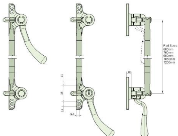
Dimensions Inward Opening 4 hole Backplate
