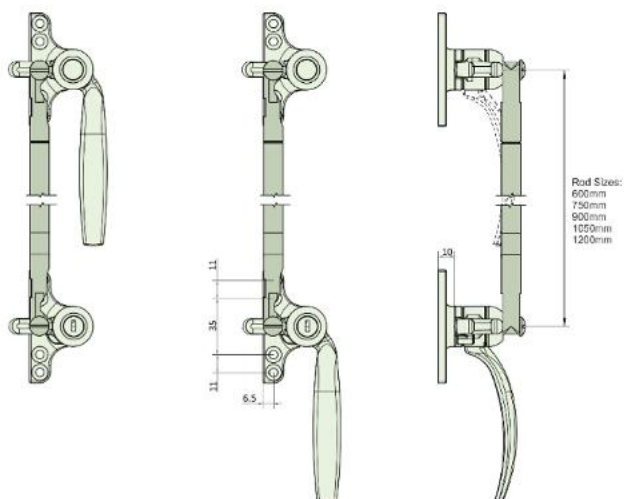
Dimensions Inward Opening 4 hole Backplate
