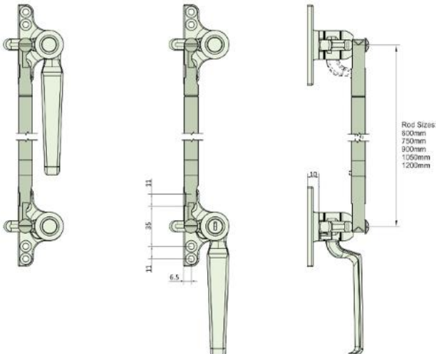
Dimensions Inward Opening 4-Hole Backplate Steel Window Fittings / Window Handles /B195/Duplex /OI
