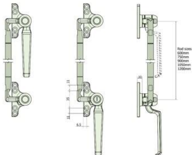
B205 Scrolled Classic Handle Duplex 4-Hole Backplate
