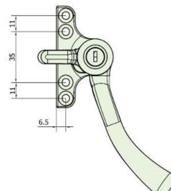
4-Hole Backplate Dimensions
