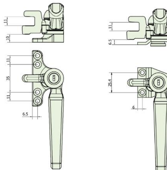
4-Hole Backplate Dimensions
