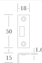
▲ AP Angle Strike Plate
