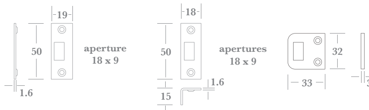
▲ FP Flat Strike Plate
