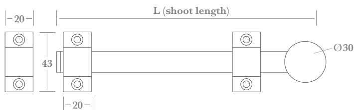
▲ 6507 shown with staple option (ST)
