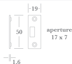
▲ FP Flat Strike Plate
