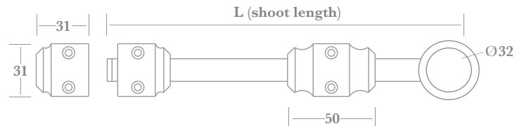
▲ 6503 shown with staple option (ST)
