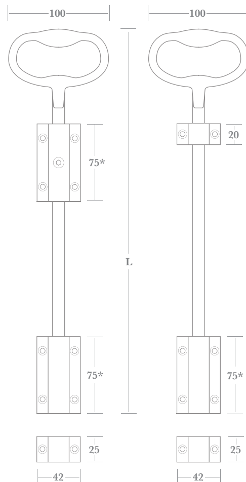
lockable version (LK)
