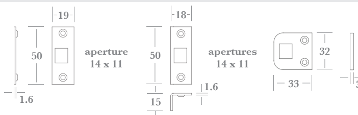
▲ FP Flat Strike Plate
